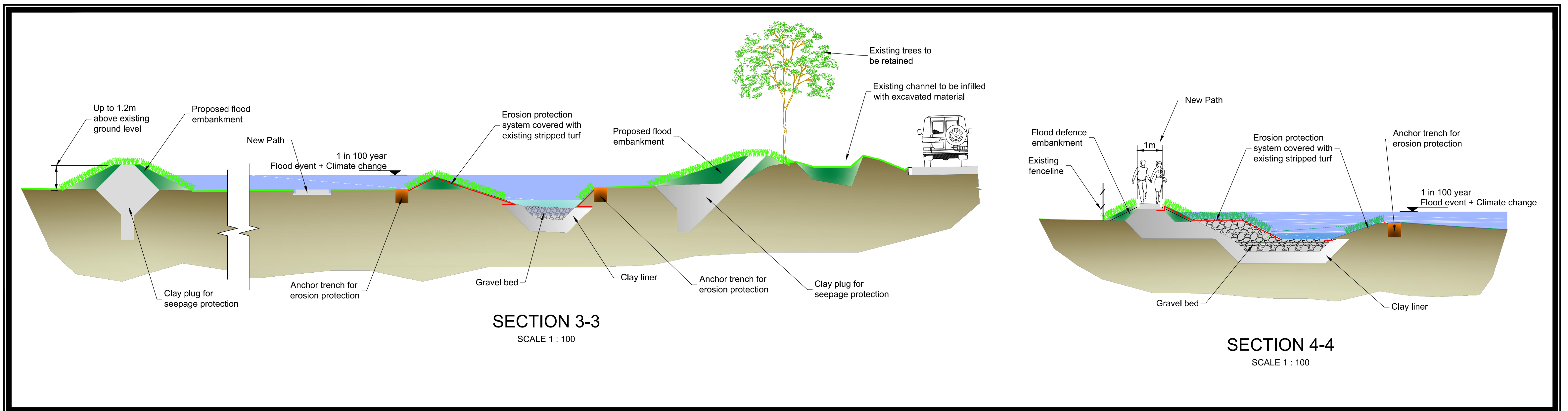
Typical Sections
